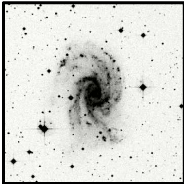
NGC2835 10'
