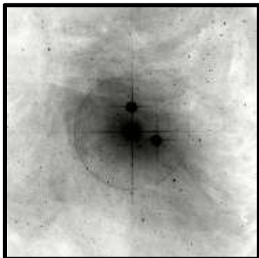
\rho Ophiuchus 25'
