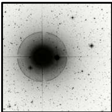
Beta 2 Capricorn
