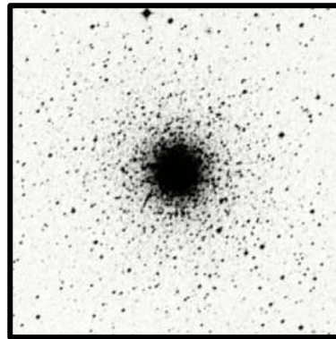
NGC5824 8'
