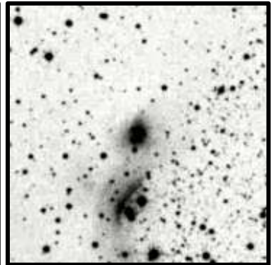
IC4954 5.0'
