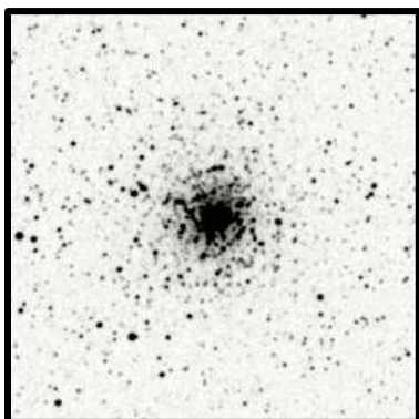
NGC6293 & NGC6294 5'
