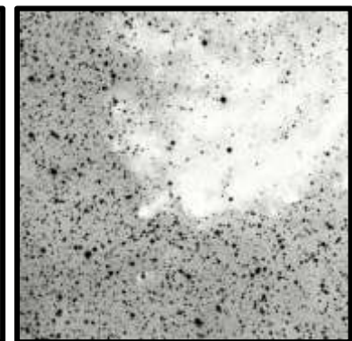
Barnard 352 15
