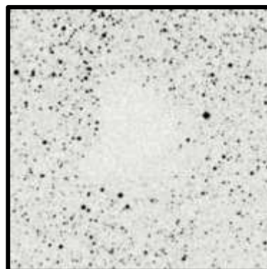
Barnard 68 10'
