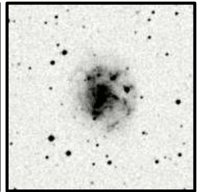
IC4536 5'
