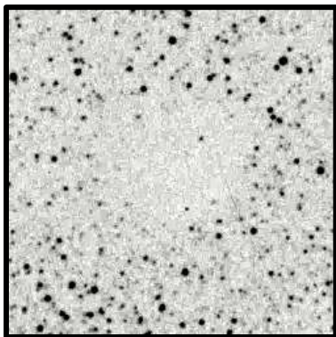
Barnard 98 7'
