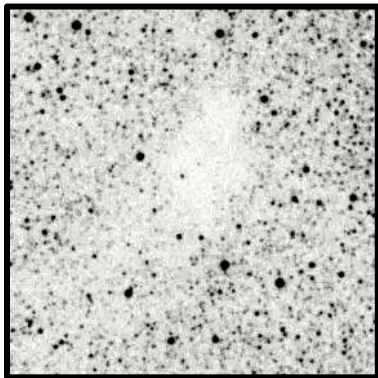
Barnard 90 8'
