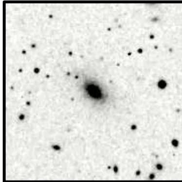
NGC5931, IC1122 5'
