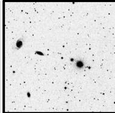
IC4562 Group 8'
