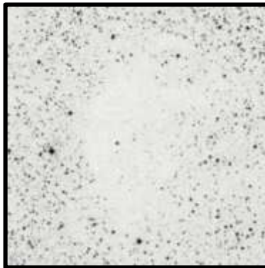
Barnard 92 20'
