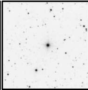
Barnard's Star 2017
