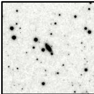
IC4617 5'
