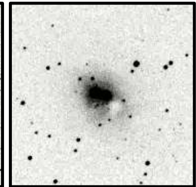
NGC6590 - IC4700 5.0'
