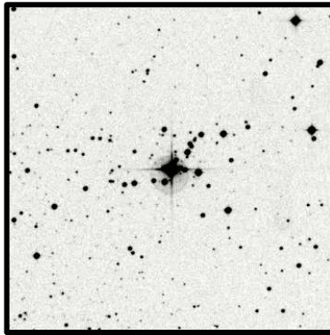
NGC6383 10'
