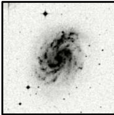
NGC5584 5'
