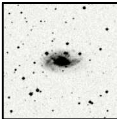
IC4999 5'
