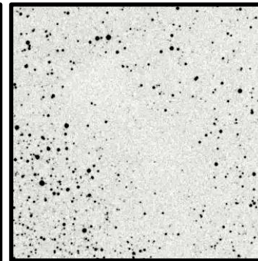
Barnard 93 10'
