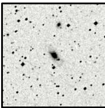
IC4537 5'
