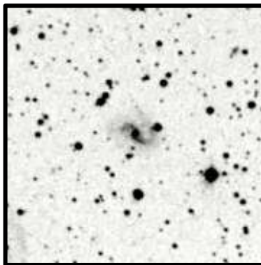
IC1296 5'
