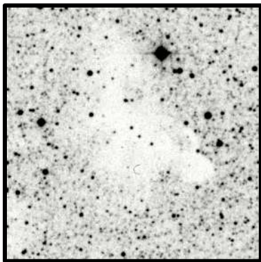
Barnard 86 8'
