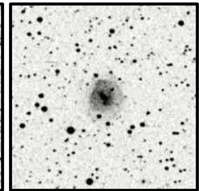
IC4688 5'
