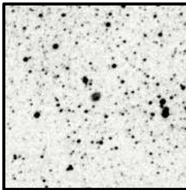
IC4673 5'
