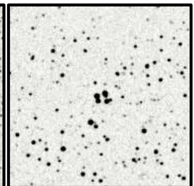
NGC6354 5'
