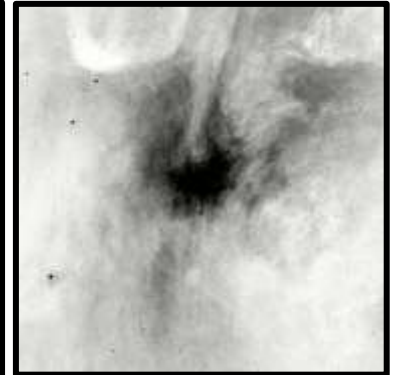
IC4603 25'
