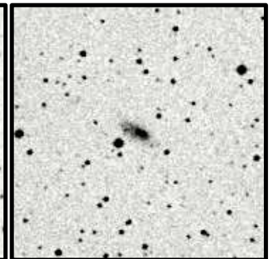
IC4627 5'
